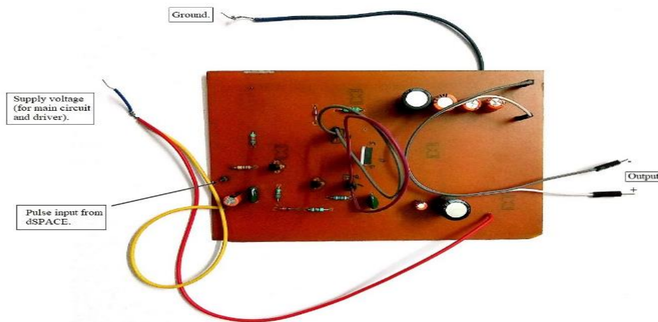
Fig. 8 The circuit implementation of the DC-DC Buck converter
