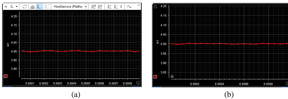
Fig. 13 Regulation of output voltage for load resistance of (a) 100\ \Omega (b) for 100\ \text{k}\Omega
