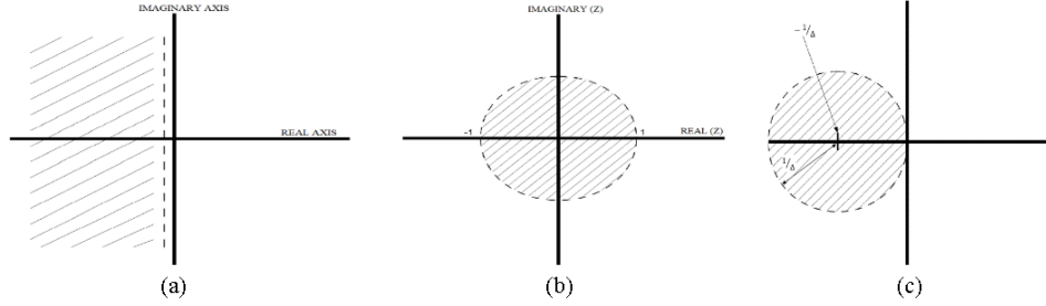
Fig. 2 (a) Stability zone: S domain, (b) Stability zone: Z domain, (c) Stability zone: \delta -domain
