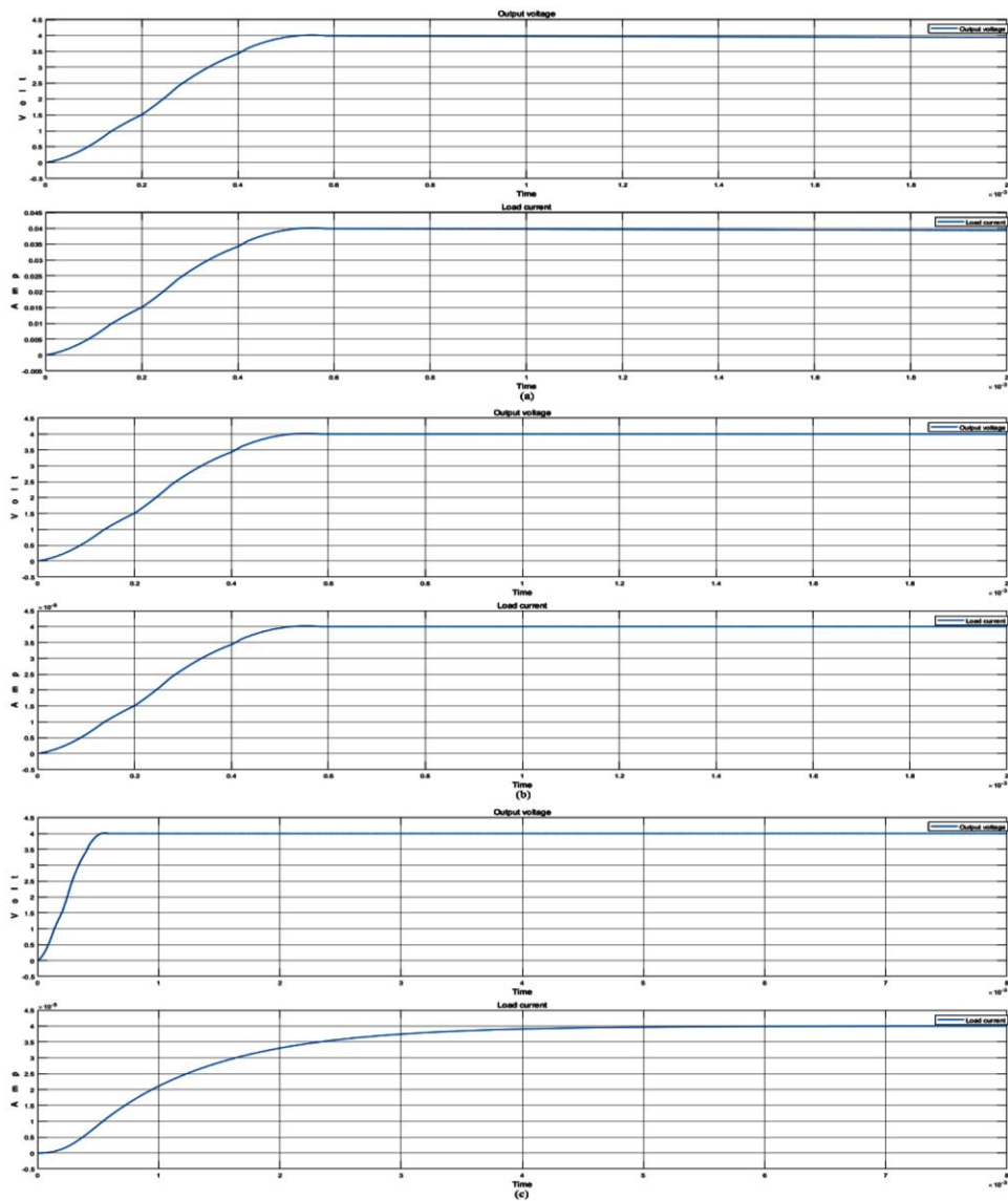
Fig. 11 Simulation of the system under different load conditions. (a) with 100 \Omega resistance, (b) with 100 k \Omega resistance, (c) with R-L load consisting of 100 k \Omega resistance and 100 H inductor
