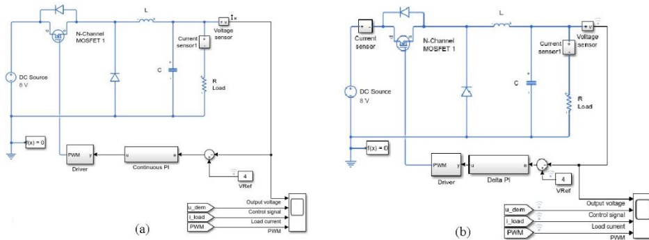
Fig. 7 Simulink model for closed-loop control of DC-DC Buck converter using (a) continuous-time PI controller with R load, (b) delta domain PI controller with R load
