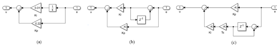
Fig. 4 (a) PI Controller in the continuous domain, (b) PI Controller in the discrete Z domain, (c) PI Controller in the discrete \delta domain
