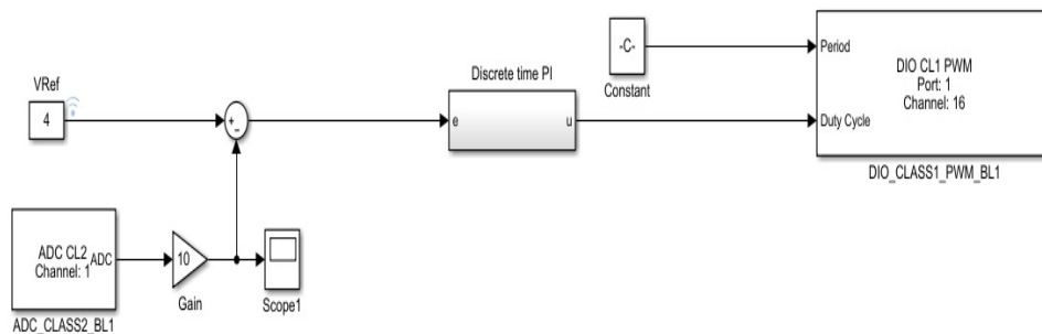
Fig. 9 Discrete PI controller in the delta-domain with dSPACE RTI blocks
