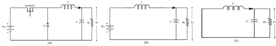
Fig. 1 (a) An ideal Buck converter, (b) Mode 1: Switch on, (c) Mode 2: Switch off
