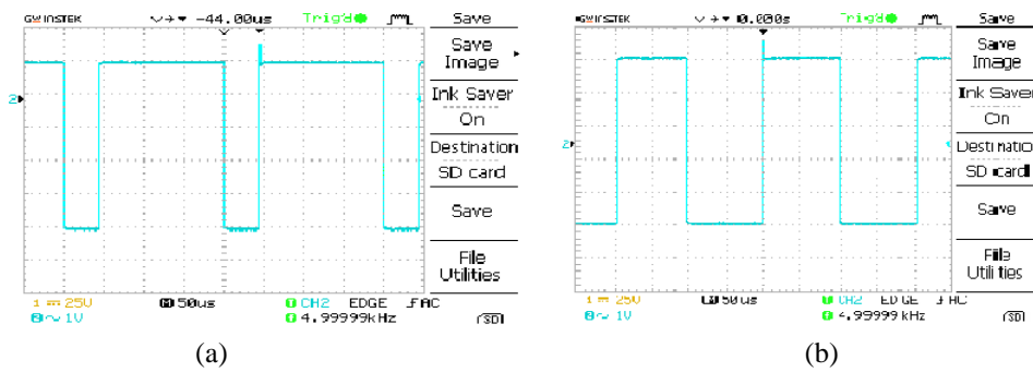
Fig. 15 PWM Signal fed to the Buck converter at (a) 75% duty cycle, (b) 50% duty cycle
