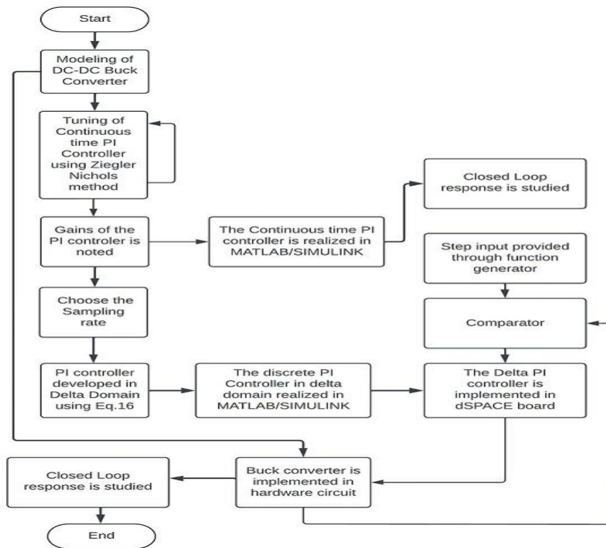
Fig. 5 Flowchart describing the complete mechanism of controller design in the delta domain
