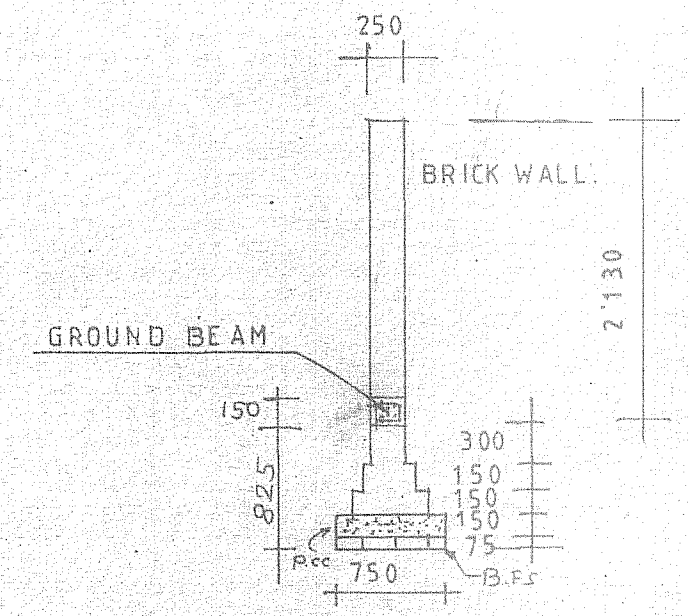
DETAILS OF BOUNDARY WALL FOUNDATION
