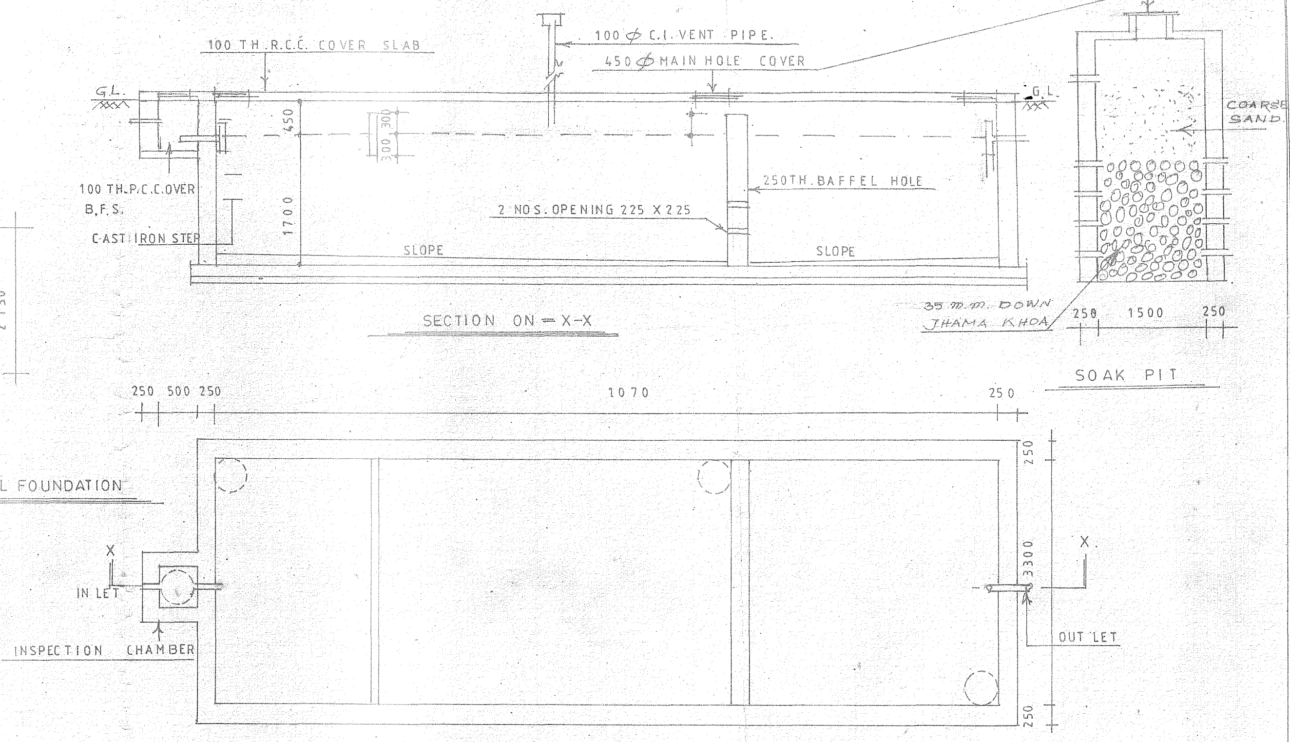
PLAN DETAILS OF SEPTIC TANK FOR 300 PERSON.
