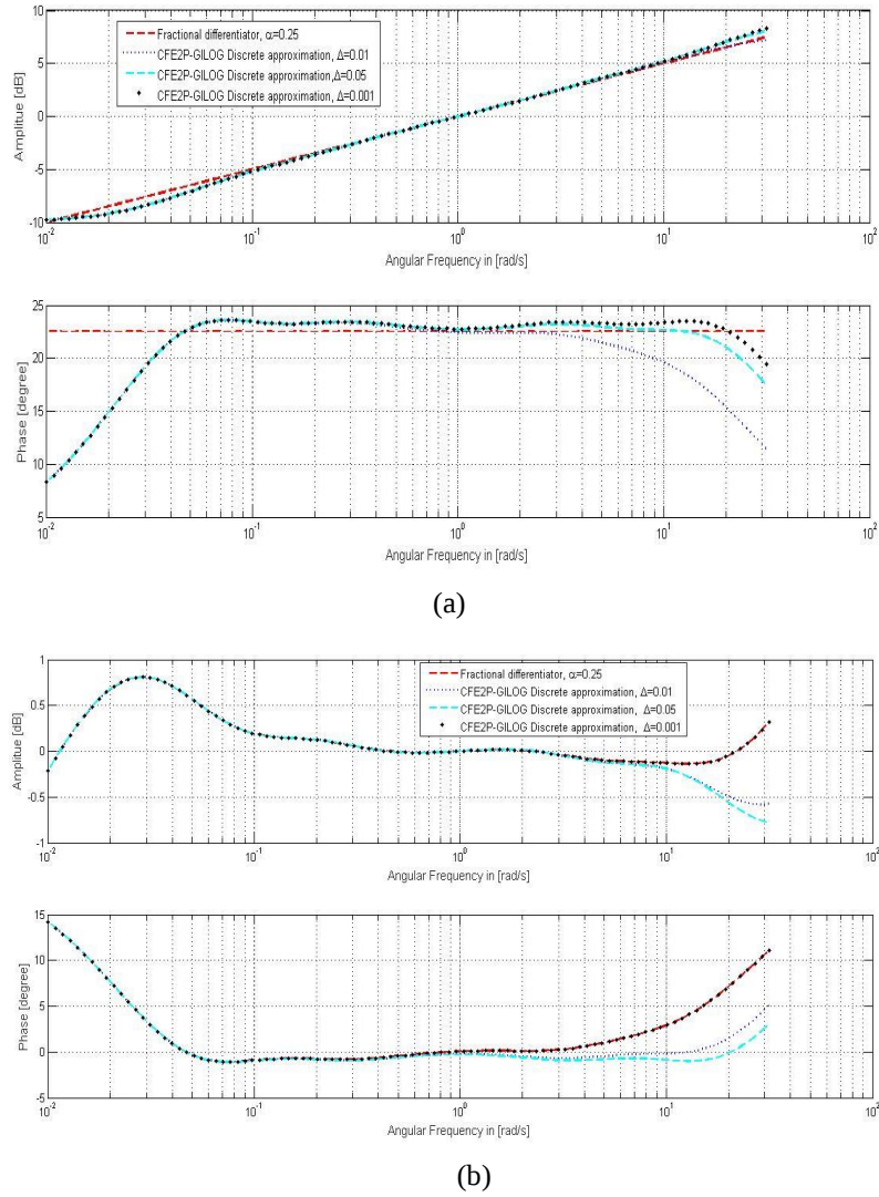
Fig. 2 a) Frequency response of G(s, 0.25) and G_{3rd}(\gamma, 0.25) for sampling rates of \Delta = 0.05 sec, \Delta = 0.01 sec and \Delta = 0.001 sec; b) Errors in approximations
