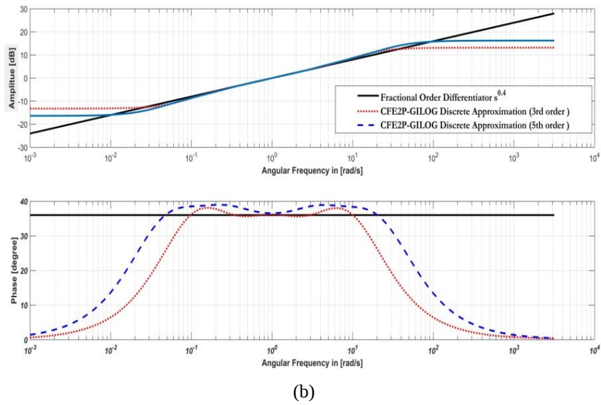
Fig. 3 a) Frequency response of the realization using z-domain and \gamma -domain for \alpha = 0.4 with \Delta = 0.001 sec; b) Fréquency responses of G(s, 0.4) , G_{3rd}(\gamma, 0.4) and G_{5rd}(\gamma, 0.4) at \Delta = 0.001 sec
