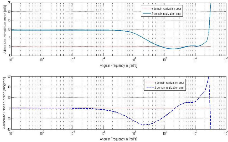
Fig. 4 Absolute errors between actual and approximated realization in z-domain and \gamma -domain
