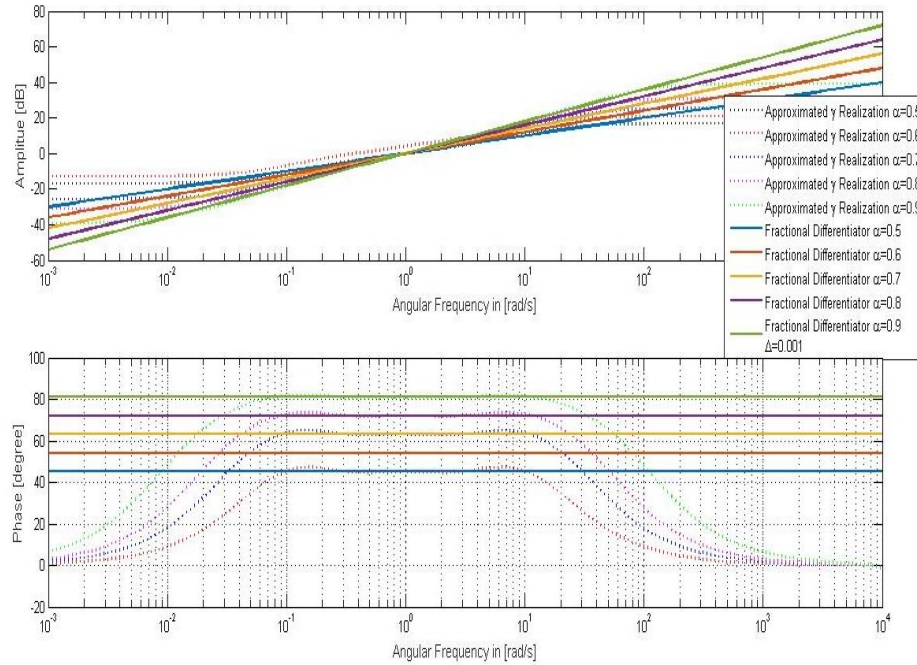
Fig. 5 Frequency response of G_{3rd}(\gamma, \alpha) for \alpha = 0.5, 0.6, 0.7, 0.8, 0.9 at \Delta = 0.001 \text{ sec}
