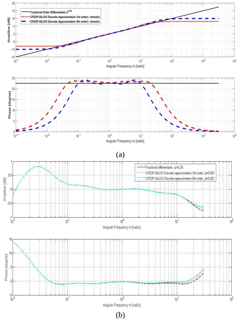
Fig. 1 a) Frequency responses of G(s,0.25) , G_{3rd}(\gamma,0.25) and G_{5th}(\gamma,0.25) at \Delta = 0.001 sec; b) Errors in approximations
